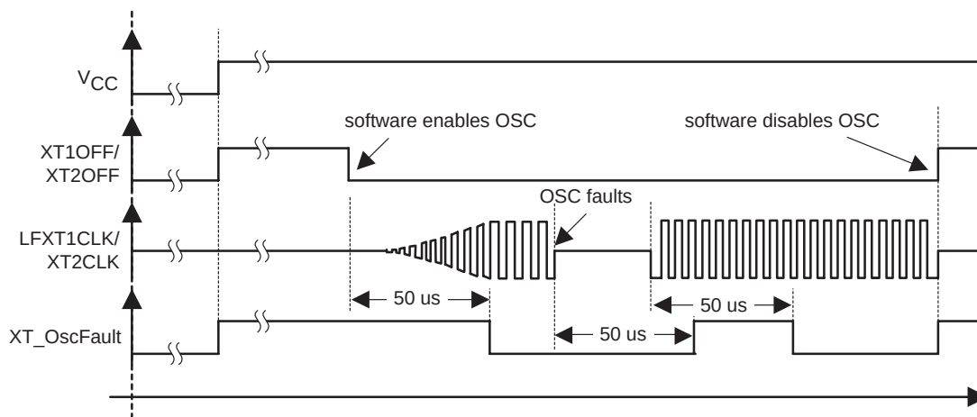
Figure 4–9. Oscillator-Fault Signal
